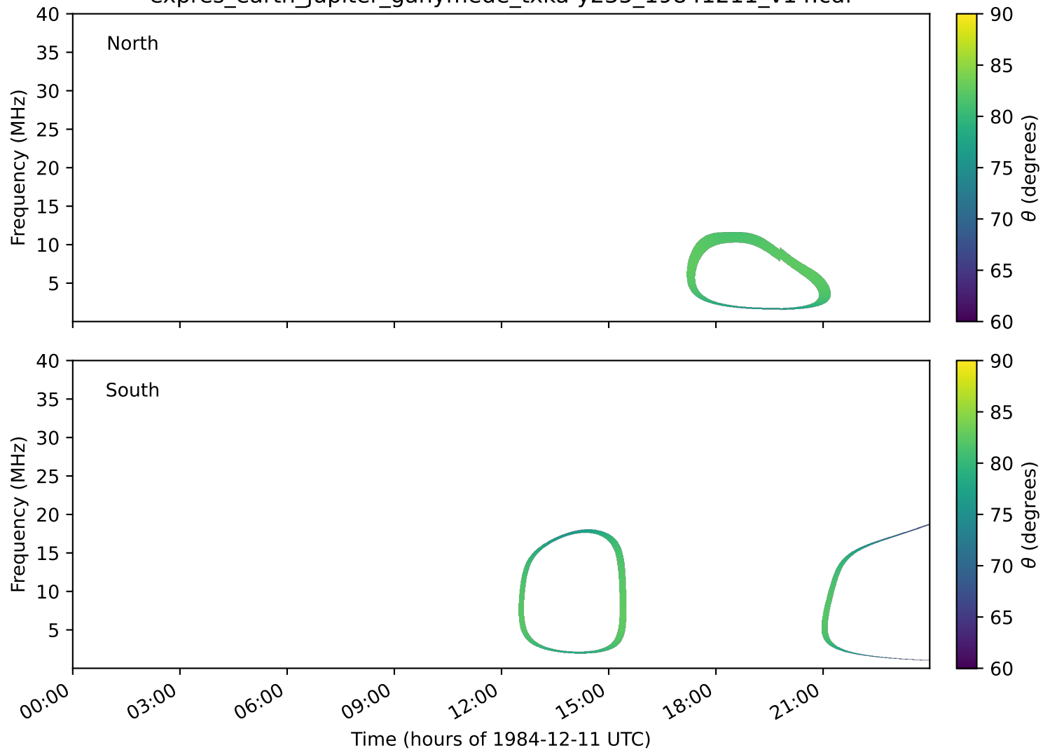
expres_earth_jupiter_ganymede_txka-y235_19841211_v14.cdf
