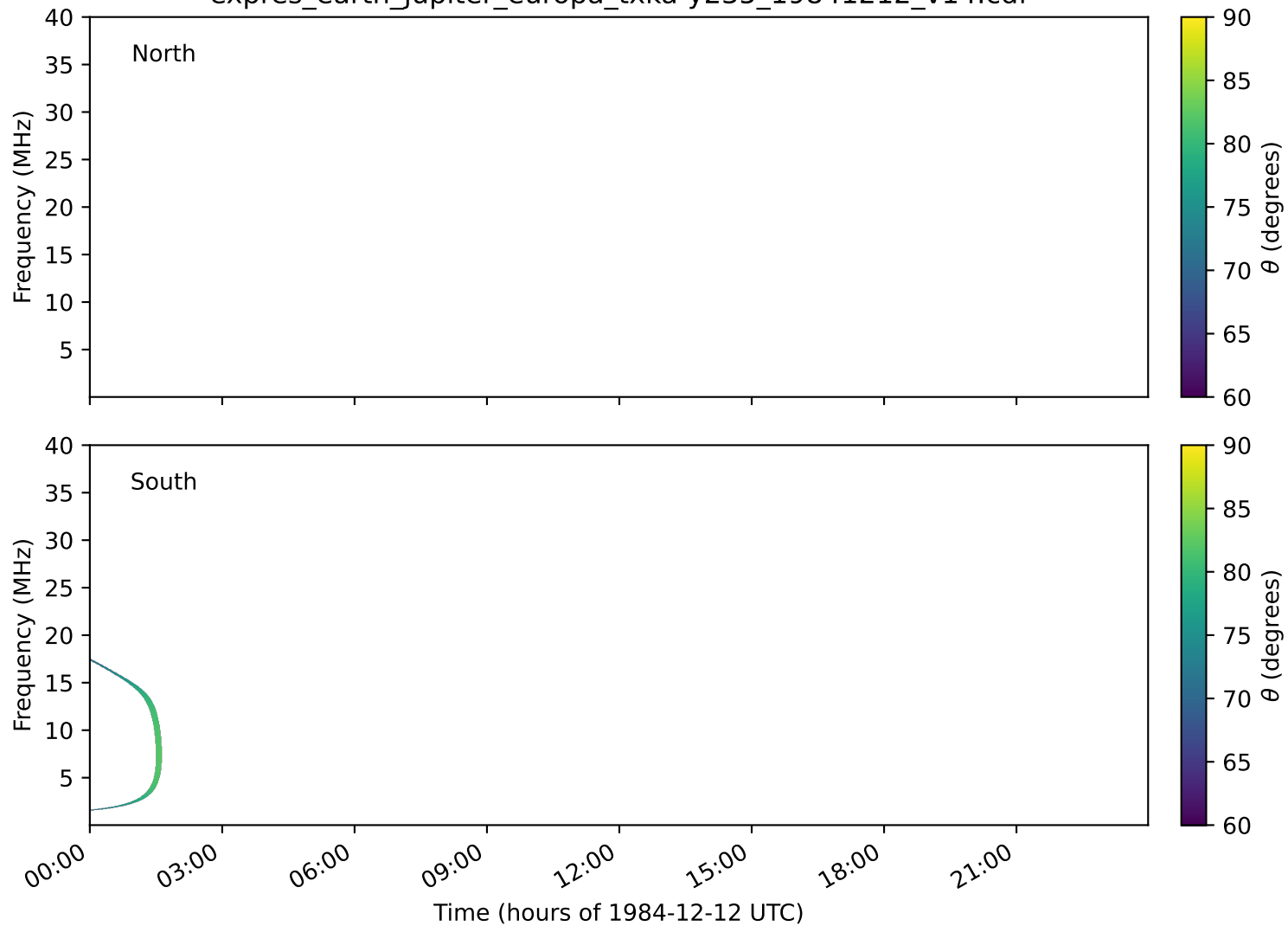
expres_earth_jupiter_europa_txka-y235_19841212_v14.cdf
