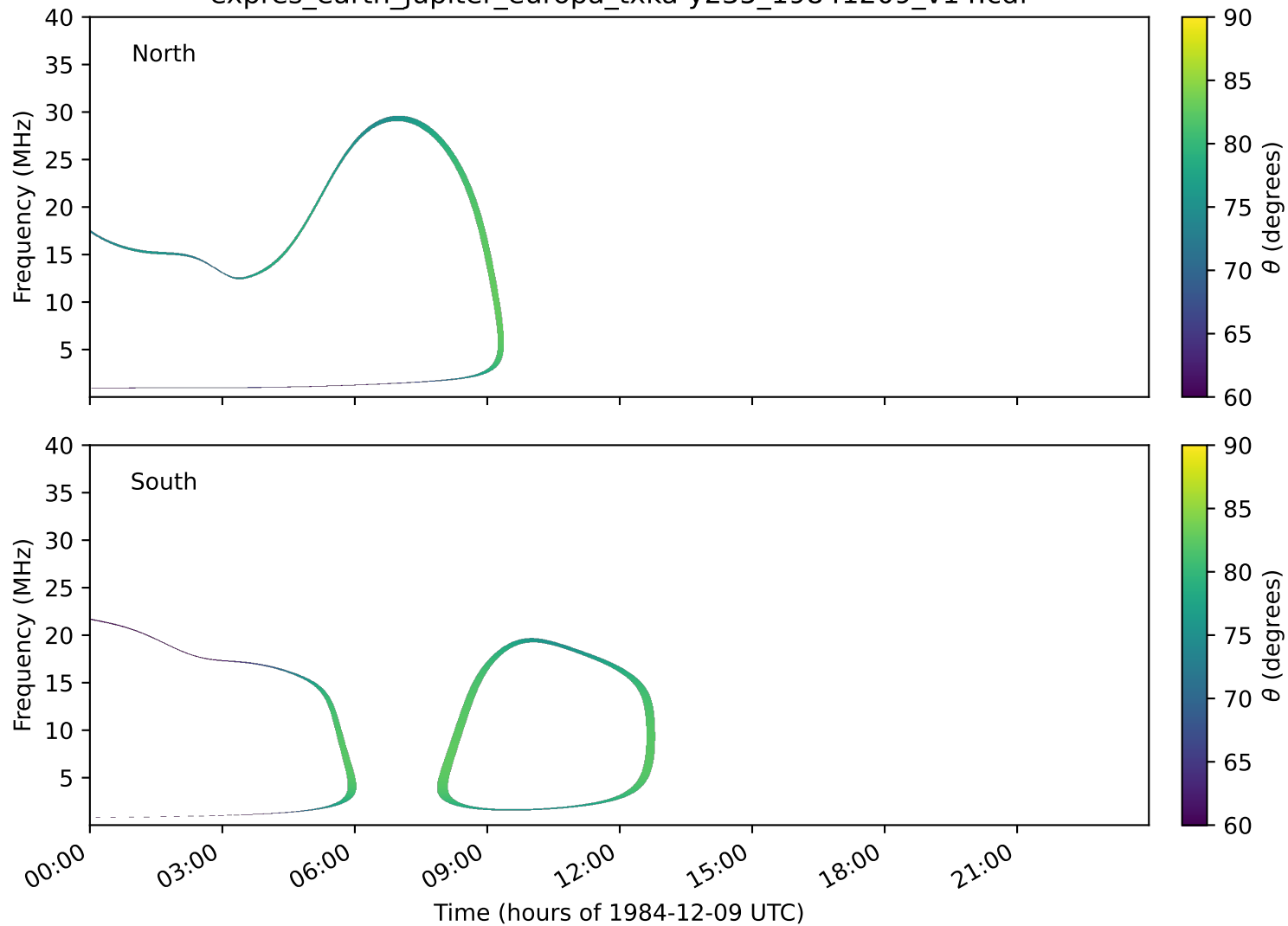
expres_earth_jupiter_europa_txka-y235_19841209_v14.cdf
