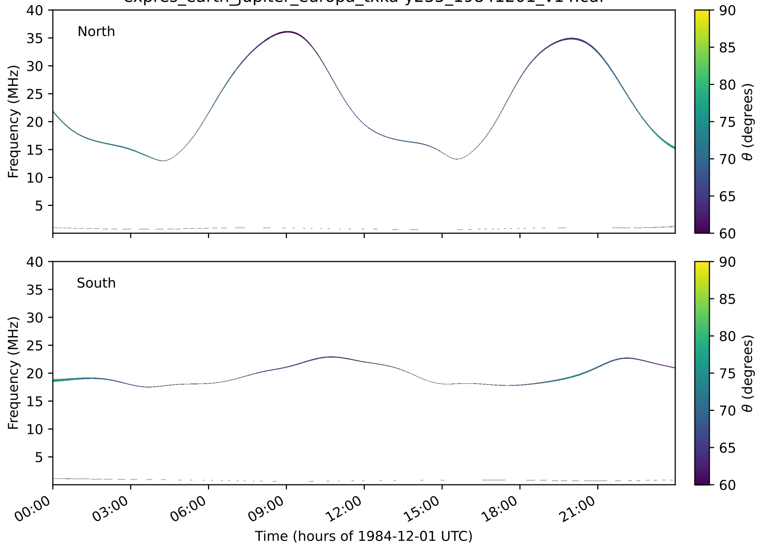
expres_earth_jupiter_europa_txka-y235_19841201_v14.cdf
