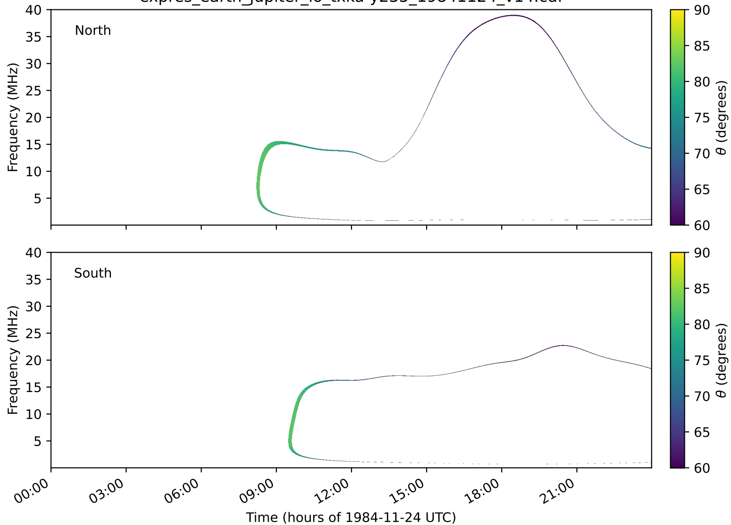
expres_earth_jupiter_io_txka-y235_19841124_v14.cdf
