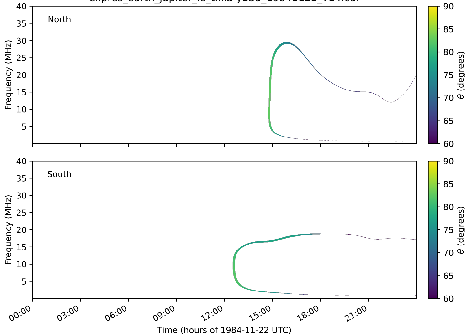
expres_earth_jupiter_io_txka-y235_19841122_v14.cdf
