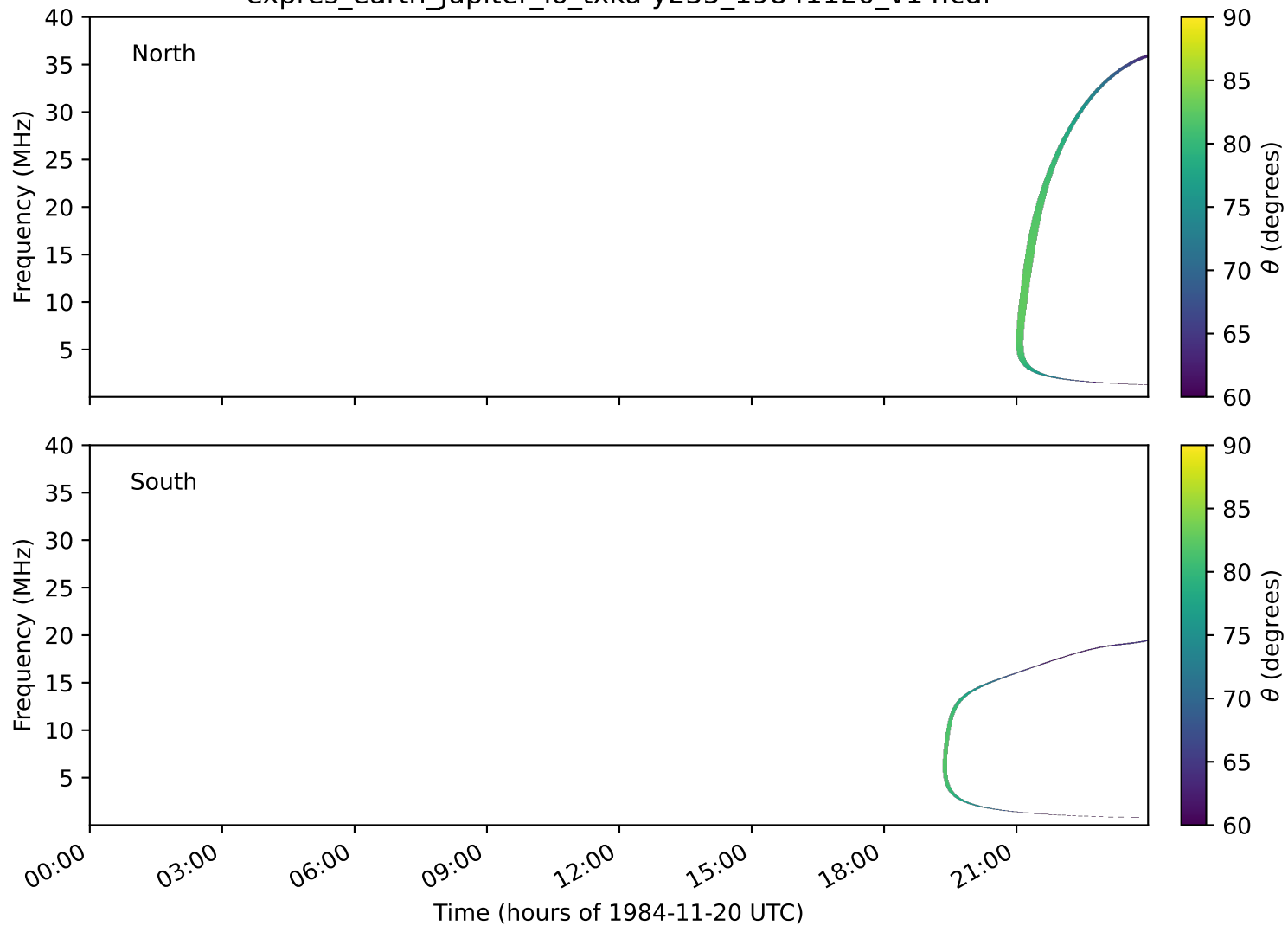
expres_earth_jupiter_io_txka-y235_19841120_v14.cdf
