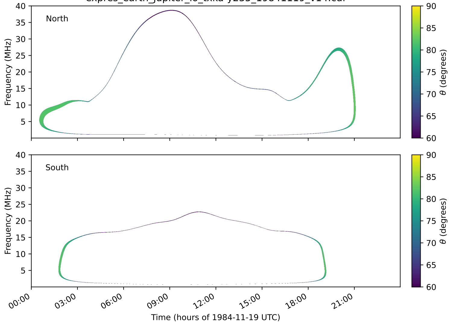
expres_earth_jupiter_io_txka-y235_19841119_v14.cdf
