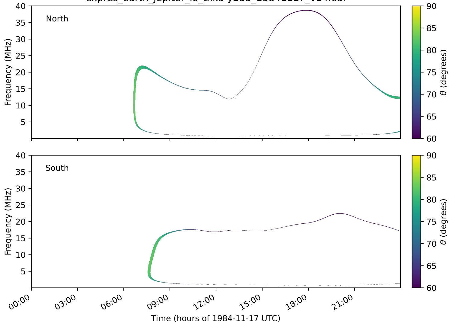
expres_earth_jupiter_io_txka-y235_19841117_v14.cdf
