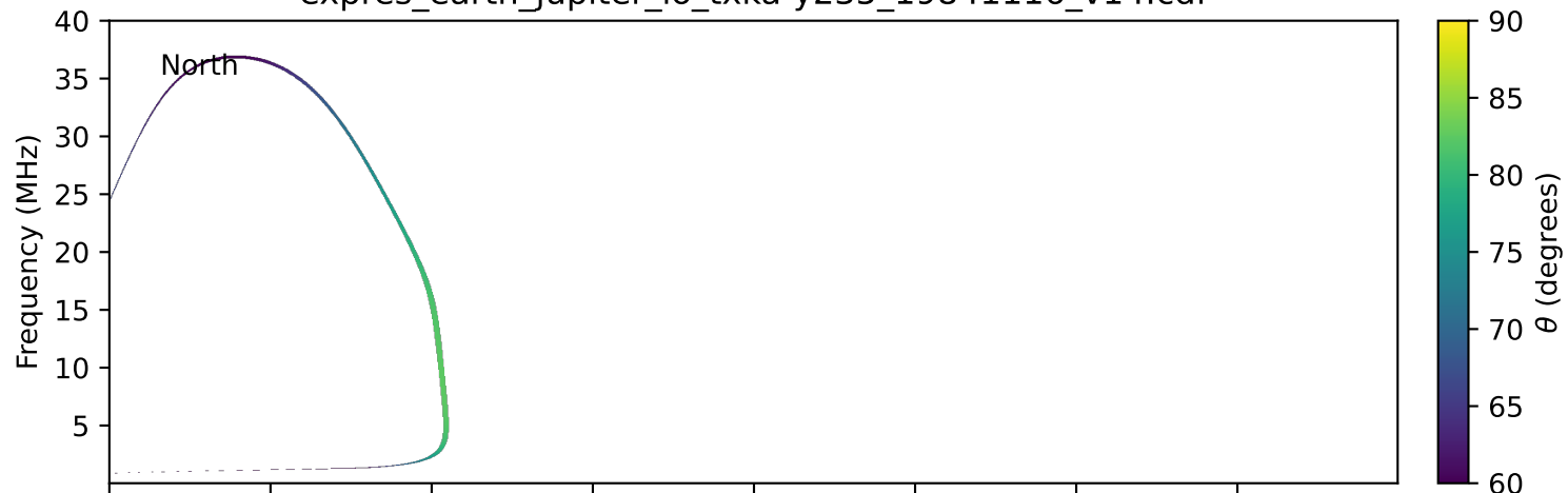
expres_earth_jupiter_io_txka-y235_19841116_v14.cdf
