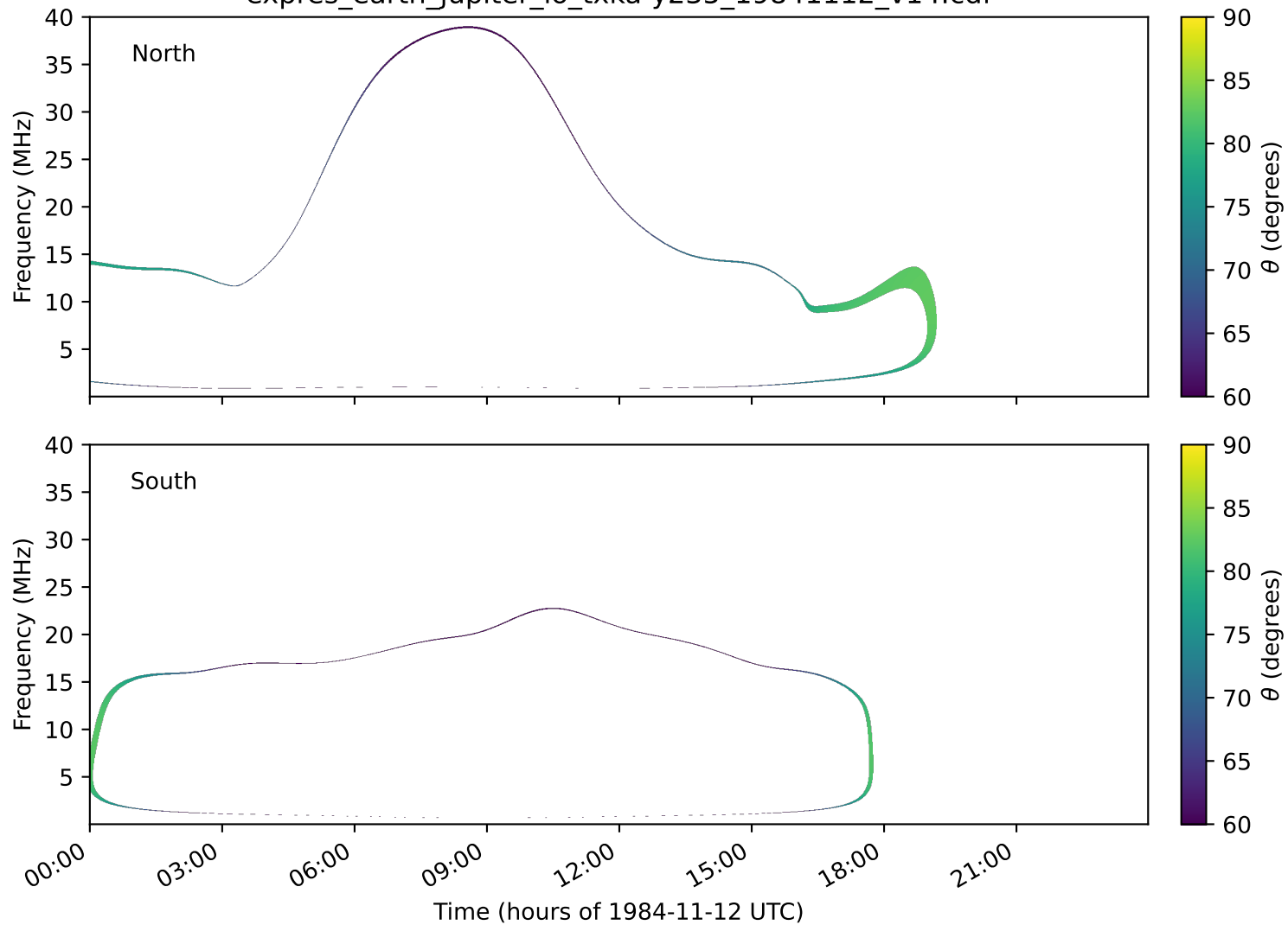
expres_earth_jupiter_io_txka-y235_19841112_v14.cdf
