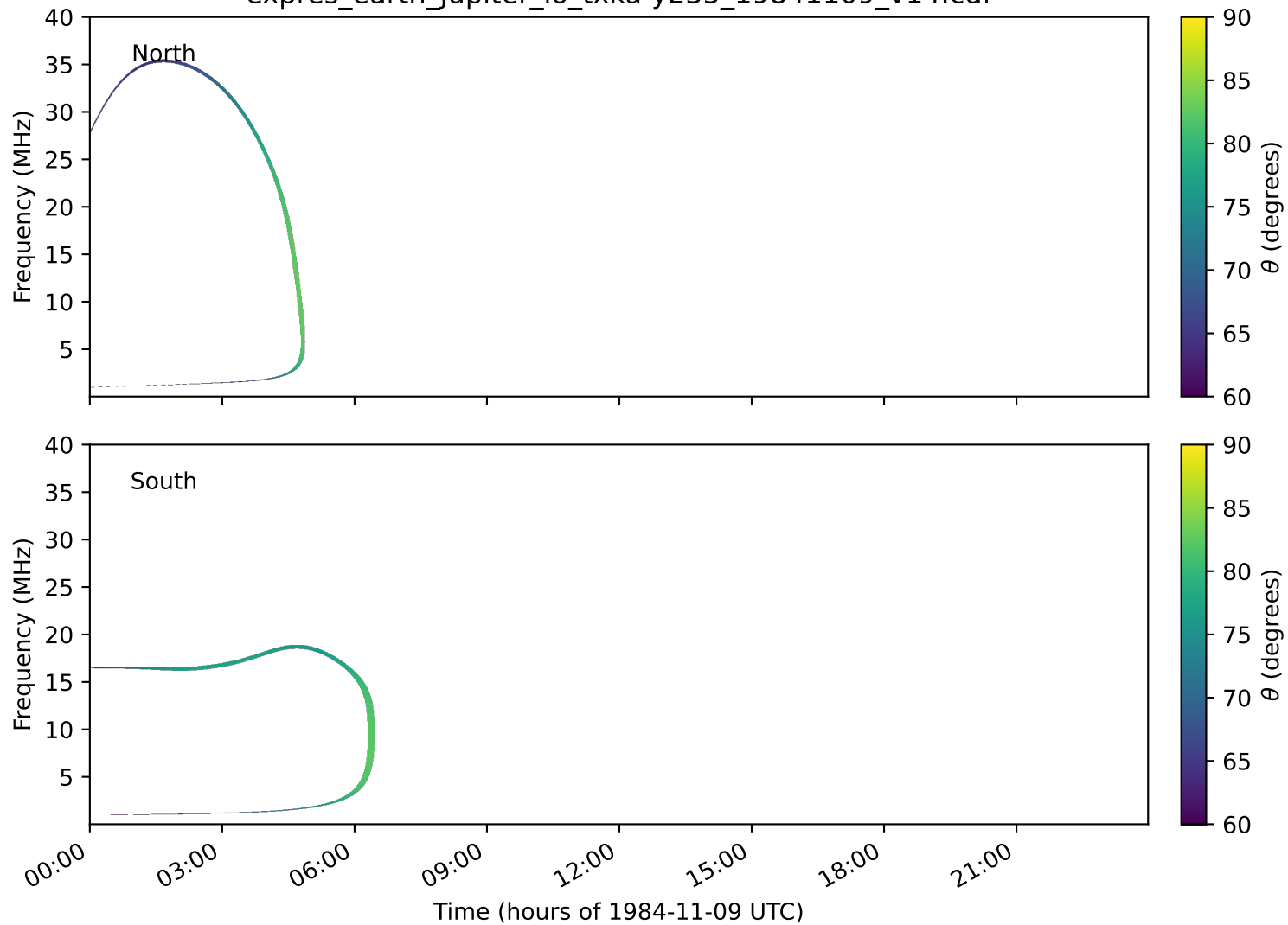
expres_earth_jupiter_io_txka-y235_19841109_v14.cdf
