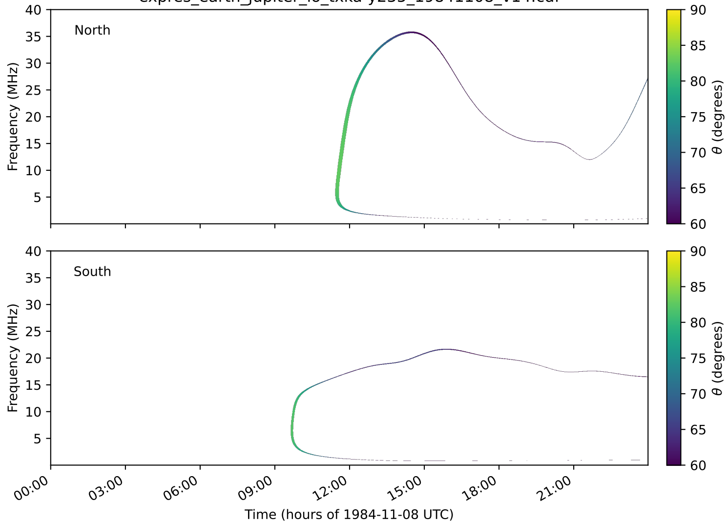
expres_earth_jupiter_io_txka-y235_19841108_v14.cdf
