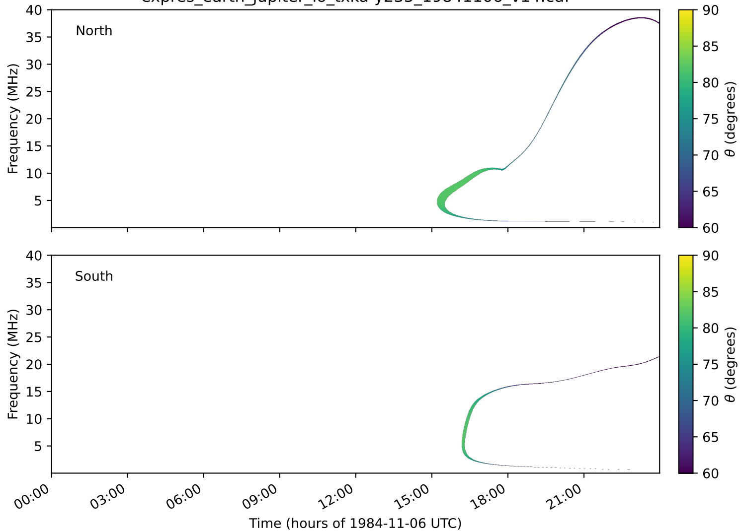
expres_earth_jupiter_io_txka-y235_19841106_v14.cdf
