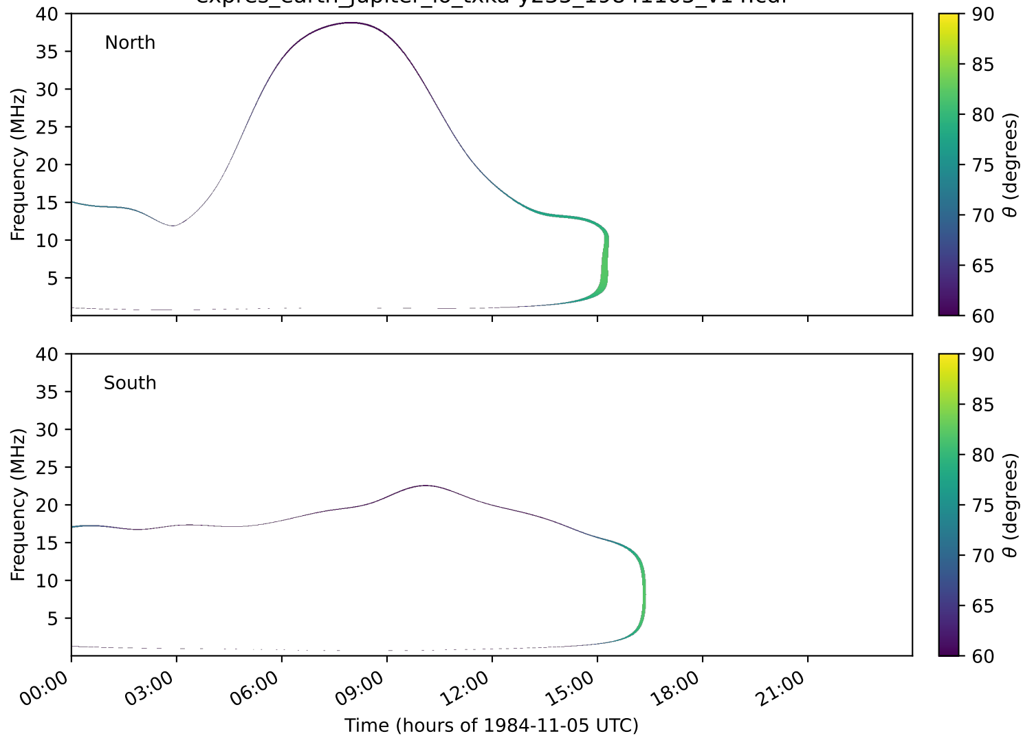
expres_earth_jupiter_io_txka-y235_19841105_v14.cdf
