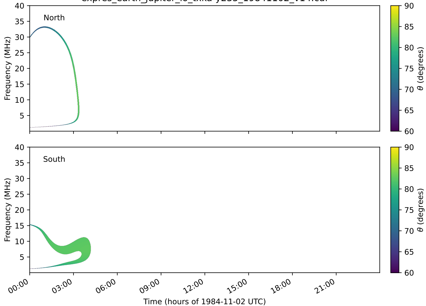
expres_earth_jupiter_io_txka-y235_19841102_v14.cdf
