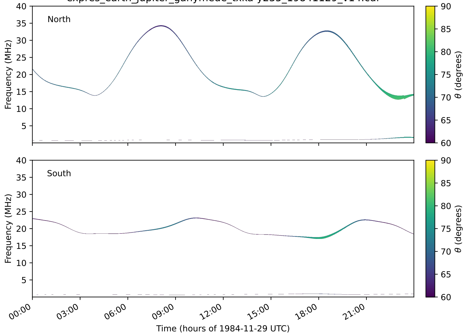
expres_earth_jupiter_ganymede_txka-y235_19841129_v14.cdf
