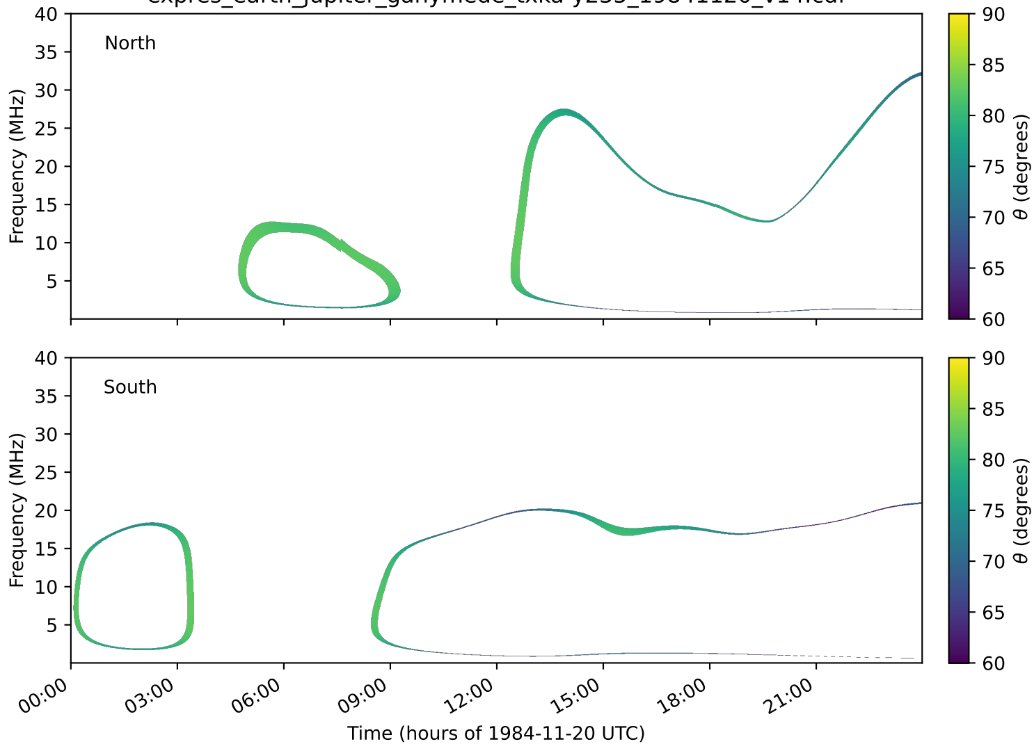
expres_earth_jupiter_ganymede_txka-y235_19841120_v14.cdf
