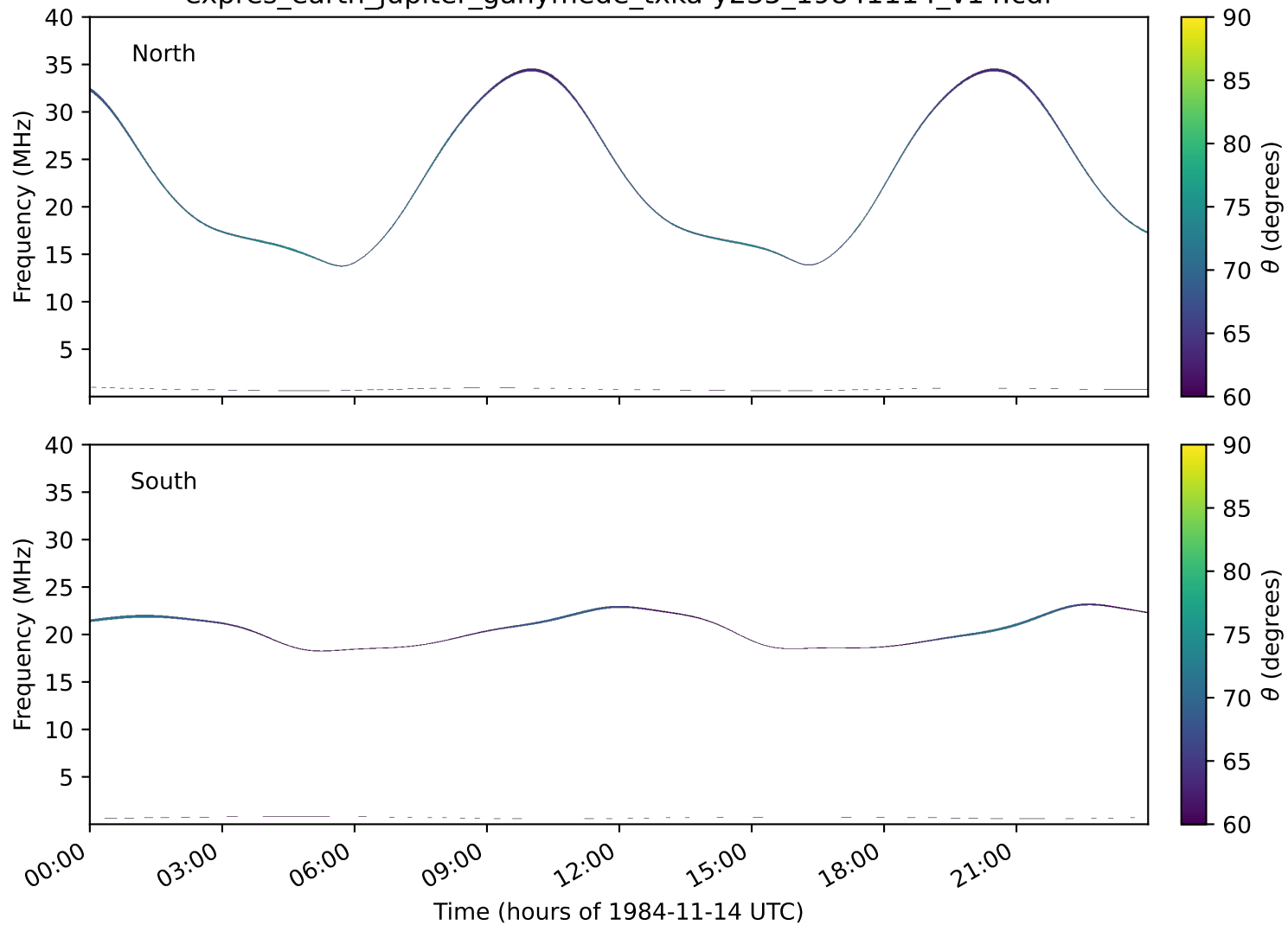
expres_earth_jupiter_ganymede_txka-y235_19841114_v14.cdf
