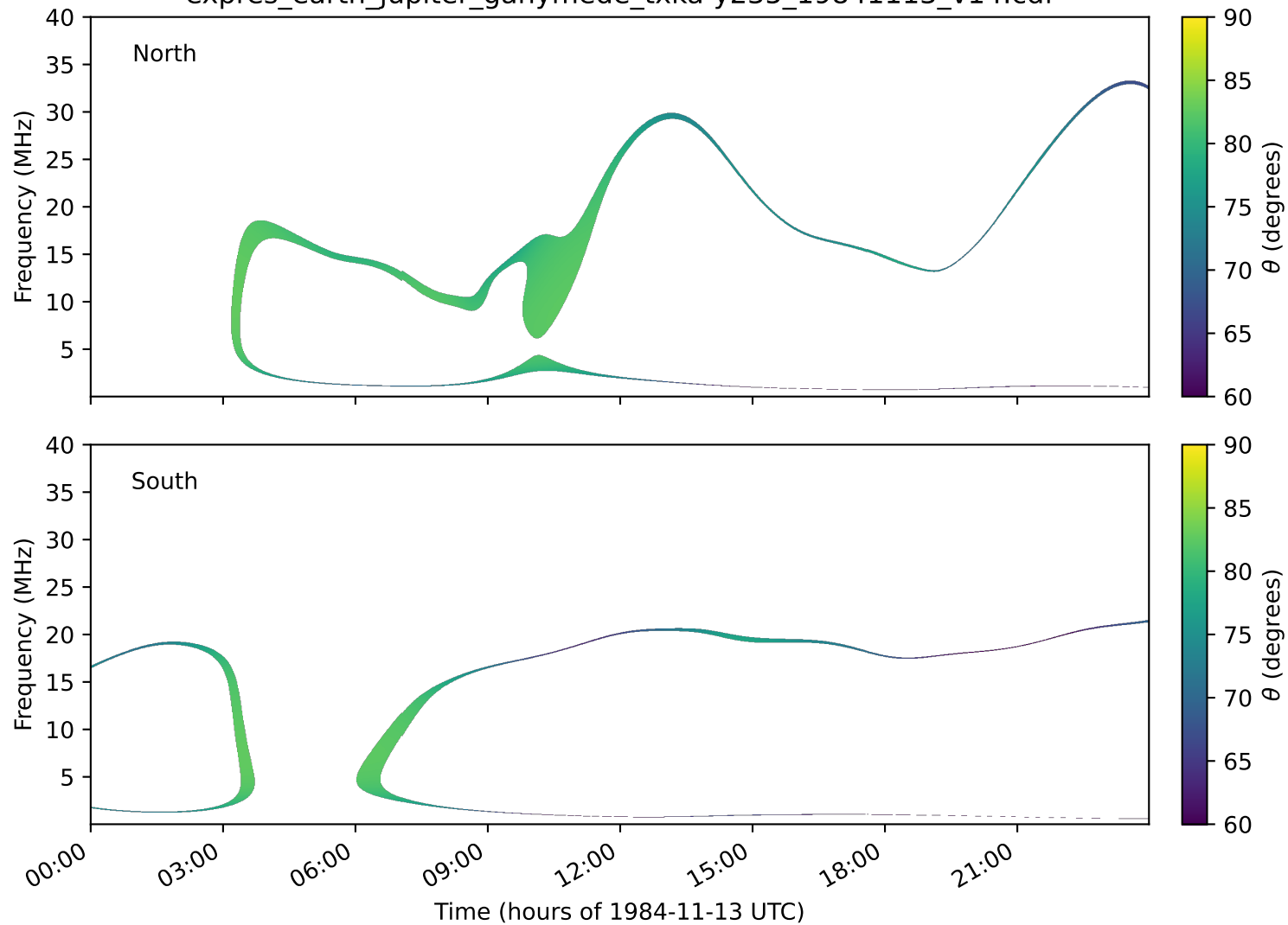
expres_earth_jupiter_ganymede_txka-y235_19841113_v14.cdf
