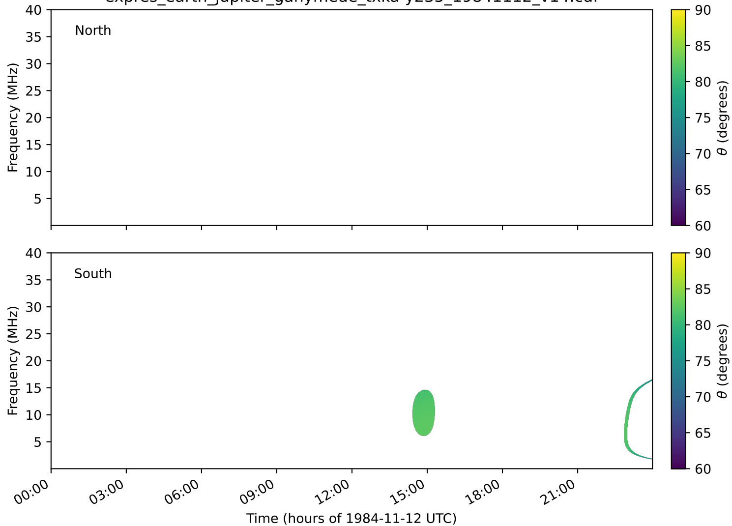
expres_earth_jupiter_ganymede_txka-y235_19841112_v14.cdf
