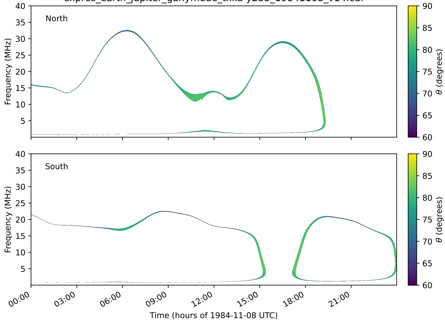
expres_earth_jupiter_ganymede_txka-y235_19841108_v14.cdf
