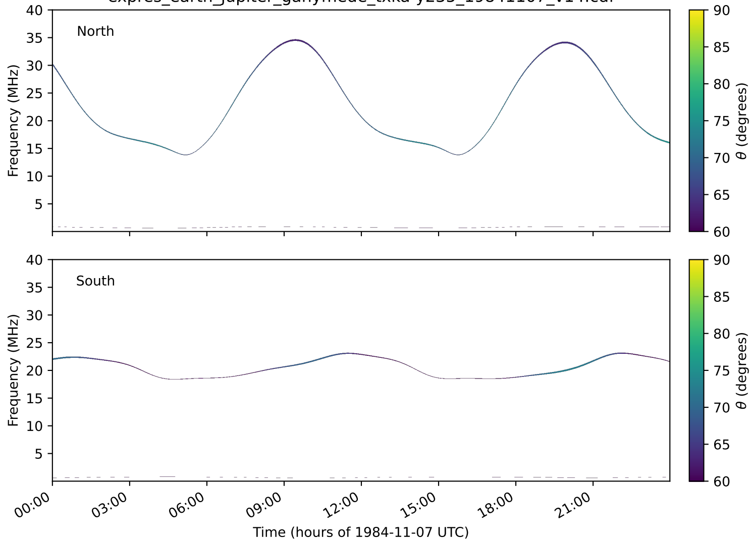
expres_earth_jupiter_ganymede_txka-y235_19841107_v14.cdf
