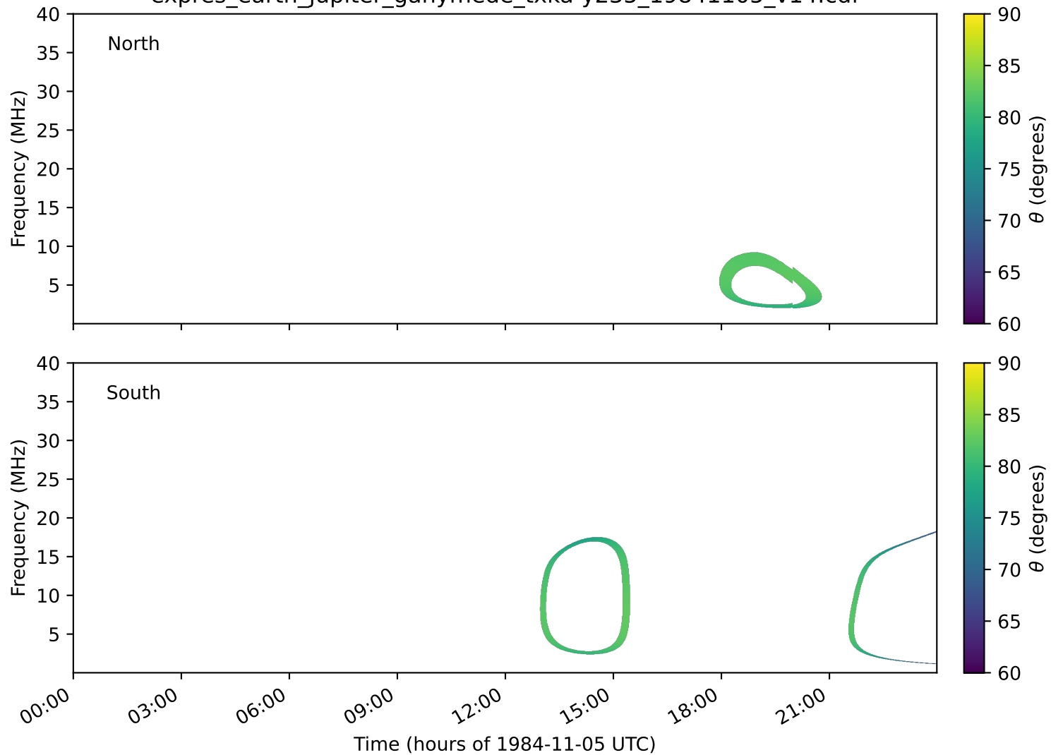
expres_earth_jupiter_ganymede_txka-y235_19841105_v14.cdf
