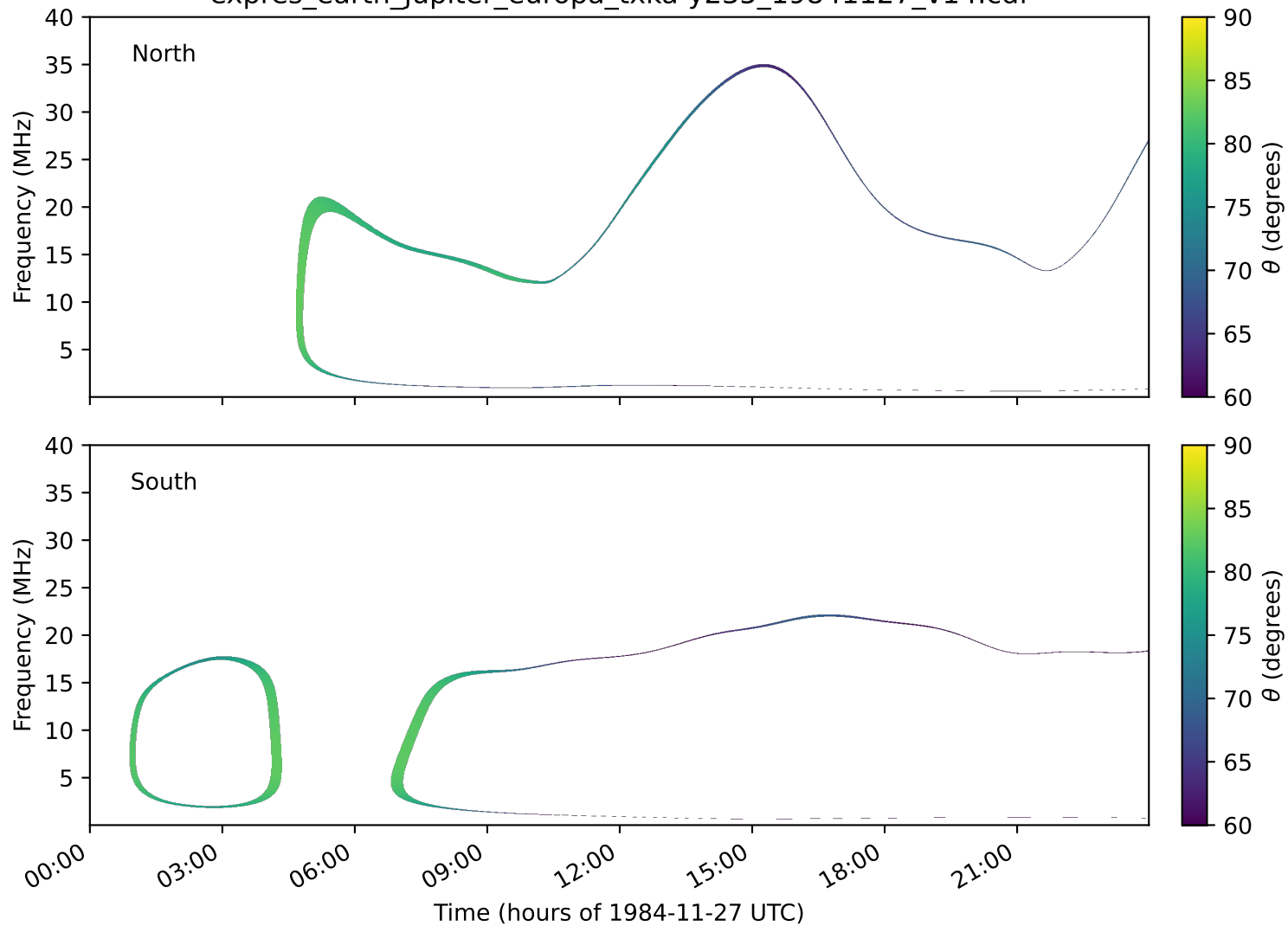
expres_earth_jupiter_europa_txka-y235_19841127_v14.cdf
