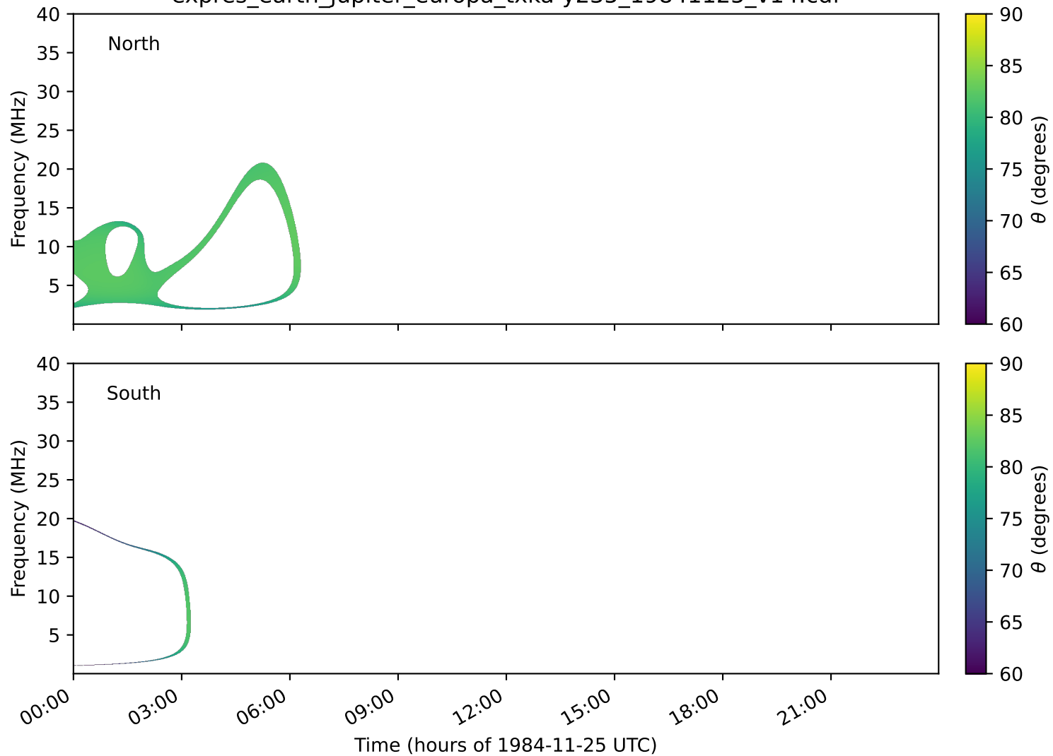
expres_earth_jupiter_europa_txka-y235_19841125_v14.cdf
