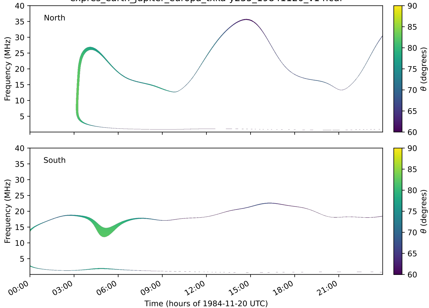
expres_earth_jupiter_europa_txka-y235_19841120_v14.cdf
