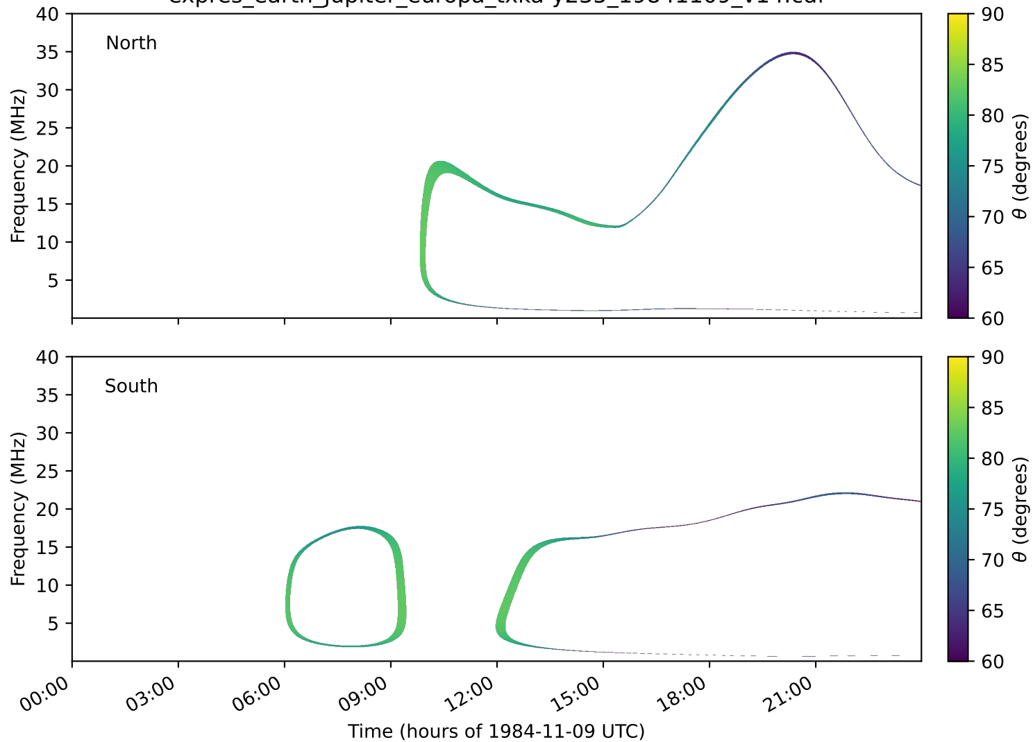
expres_earth_jupiter_europa_txka-y235_19841109_v14.cdf
