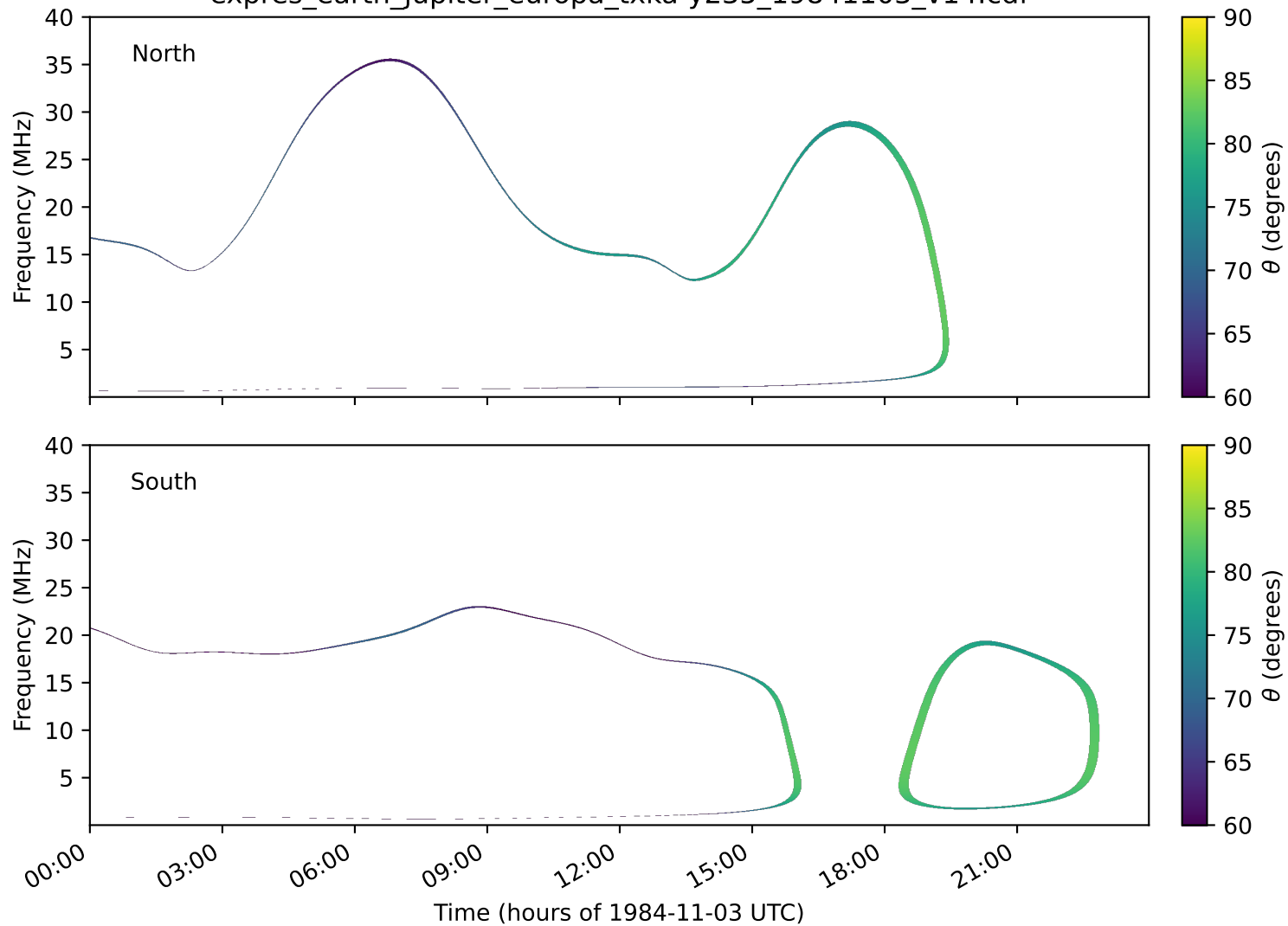
expres_earth_jupiter_europa_txka-y235_19841103_v14.cdf
