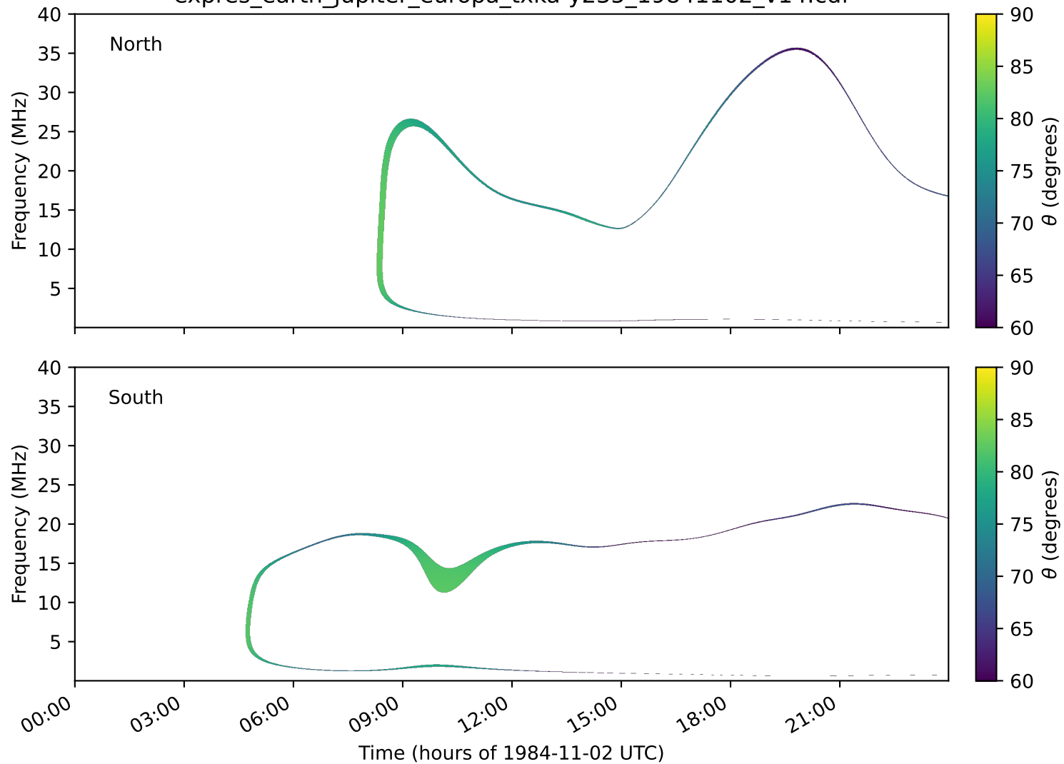
expres_earth_jupiter_europa_txka-y235_19841102_v14.cdf
