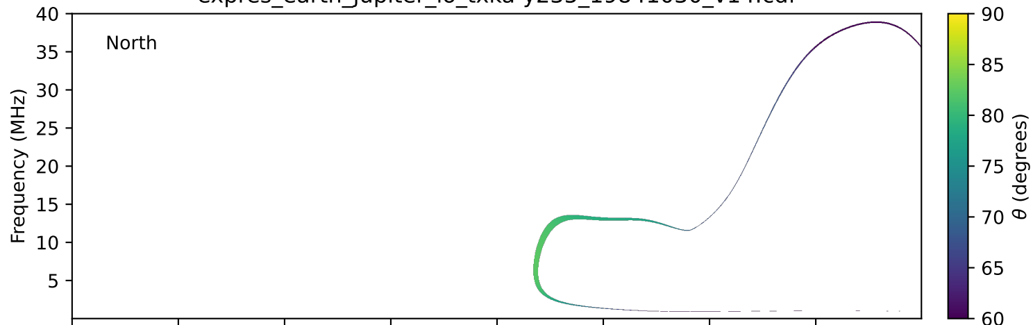
expres_earth_jupiter_io_txka-y235_19841030_v14.cdf
