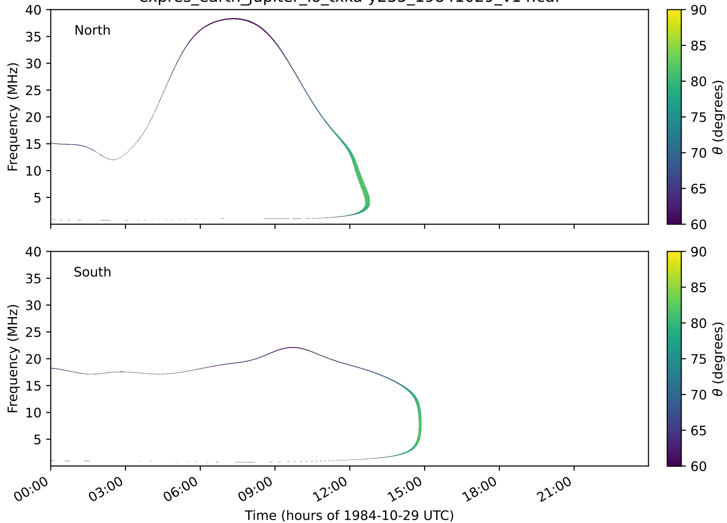
expres_earth_jupiter_io_txka-y235_19841029_v14.cdf
