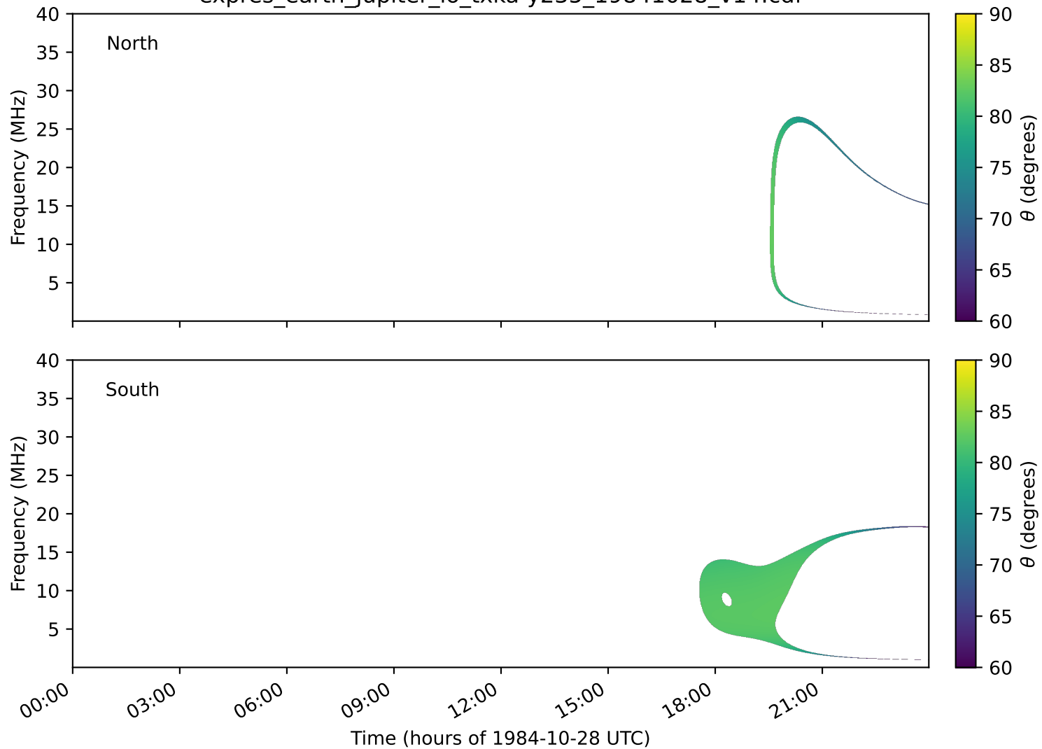
expres_earth_jupiter_io_txka-y235_19841028_v14.cdf
