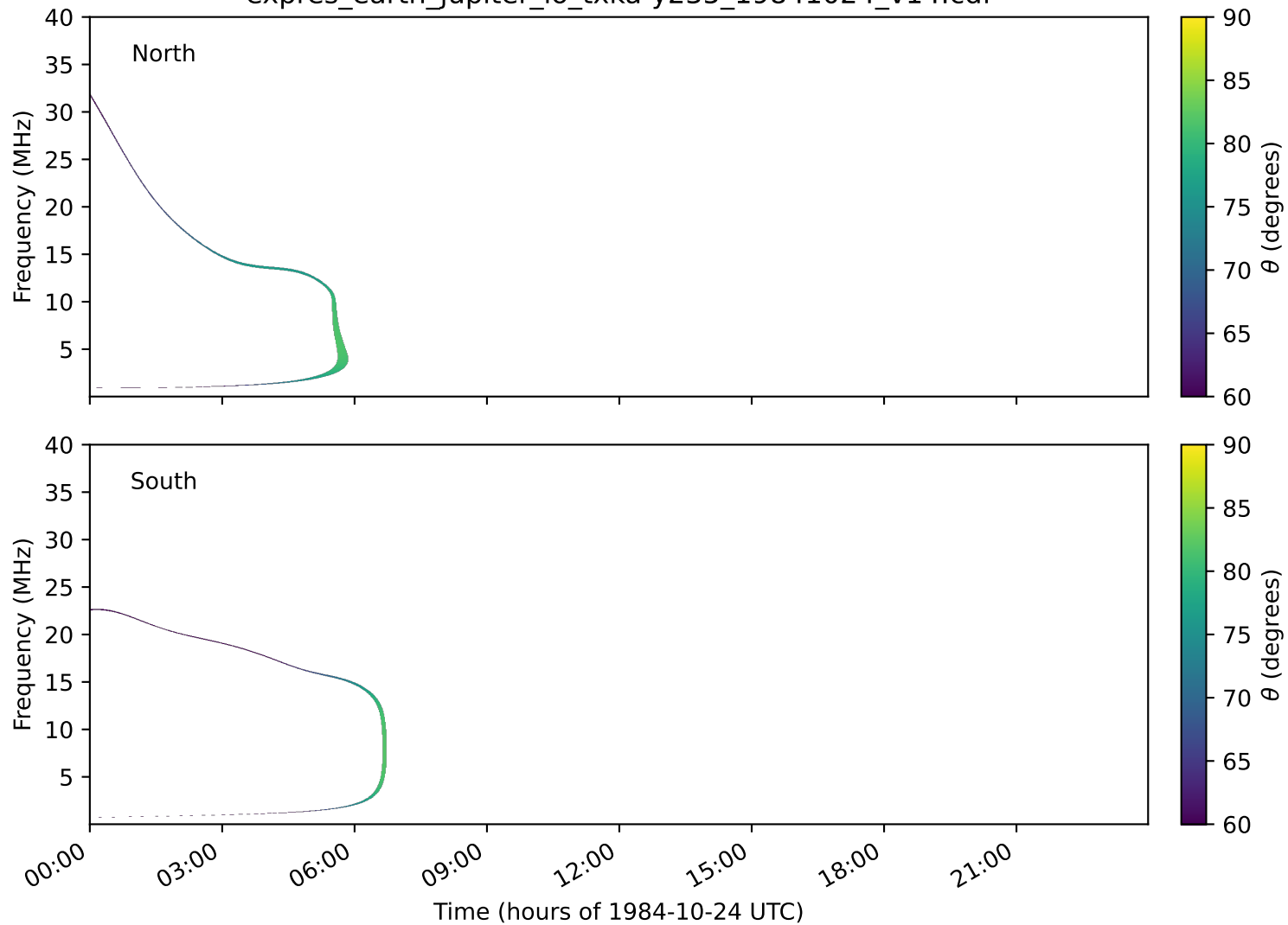
expres_earth_jupiter_io_txka-y235_19841024_v14.cdf
