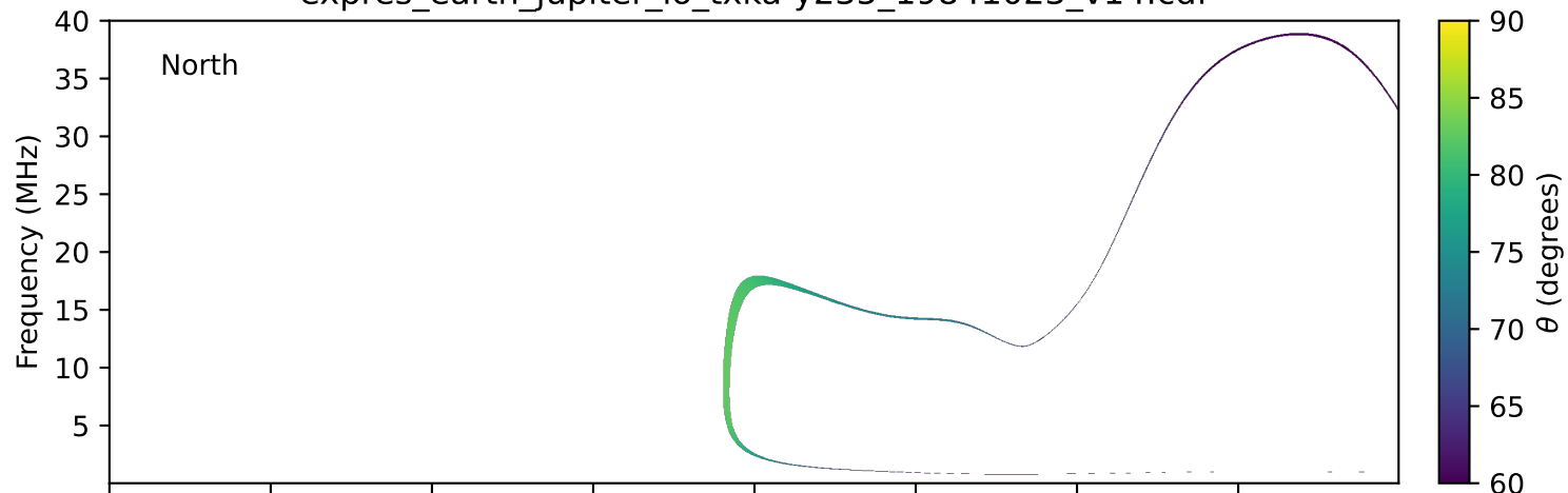
expres_earth_jupiter_io_txka-y235_19841023_v14.cdf
