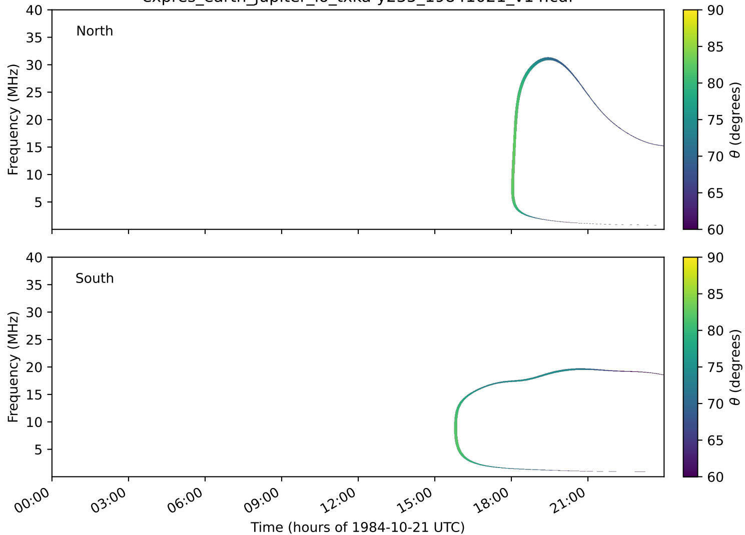
expres_earth_jupiter_io_txka-y235_19841021_v14.cdf
