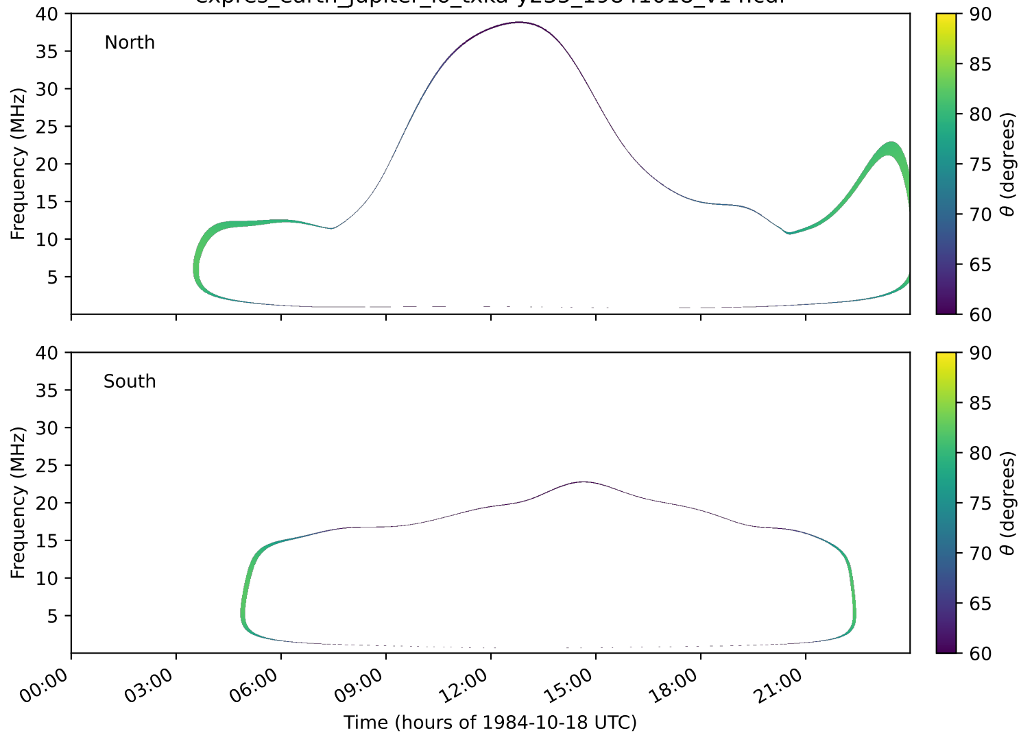
expres_earth_jupiter_io_txka-y235_19841018_v14.cdf
