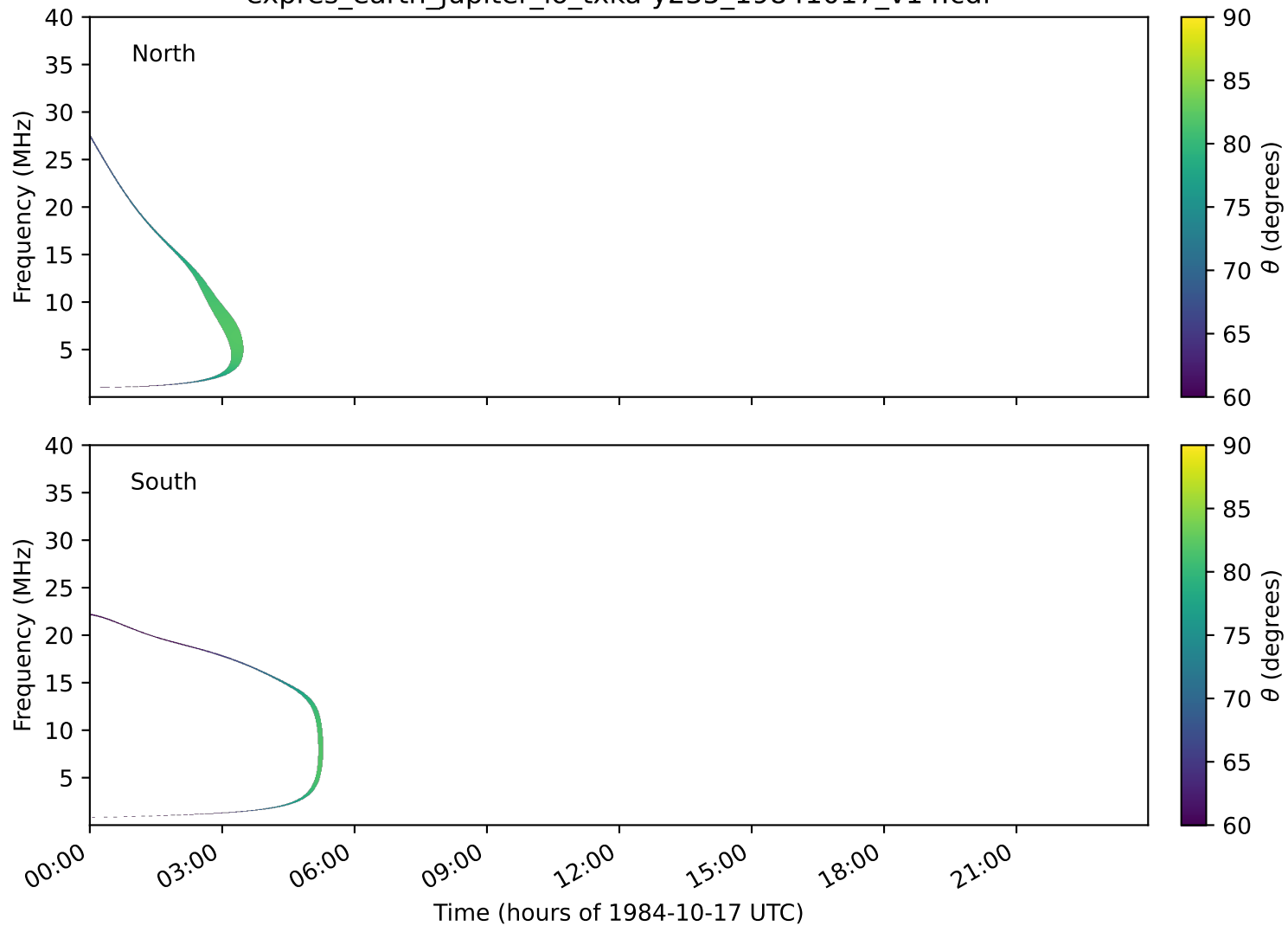
expres_earth_jupiter_io_txka-y235_19841017_v14.cdf
