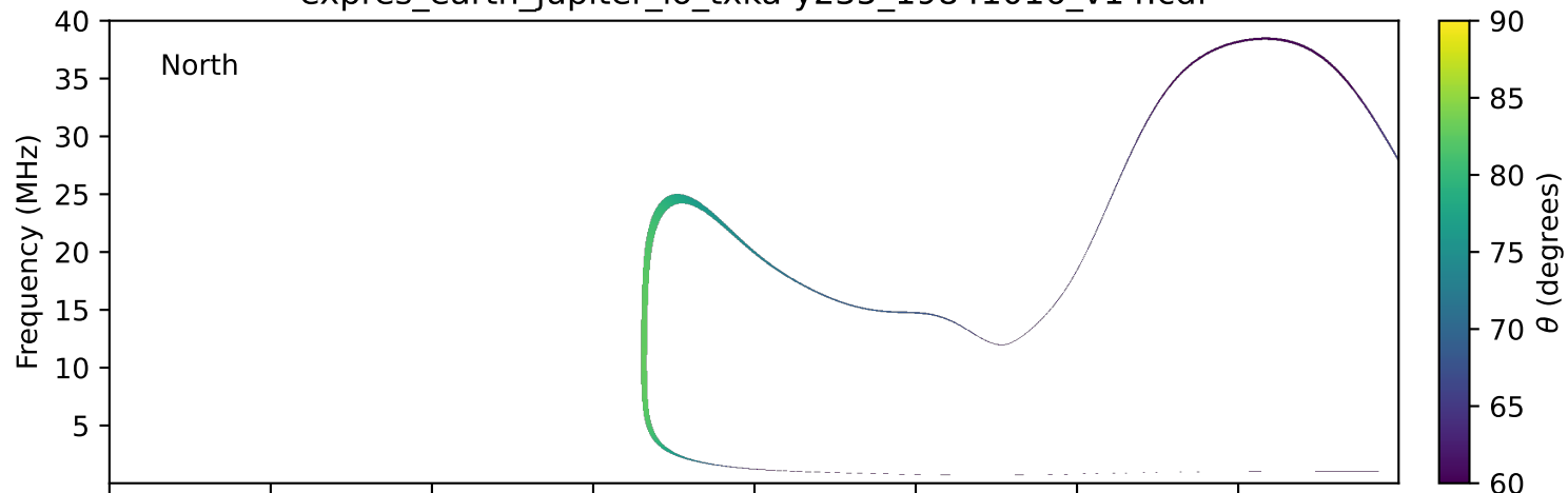
expres_earth_jupiter_io_txka-y235_19841016_v14.cdf
