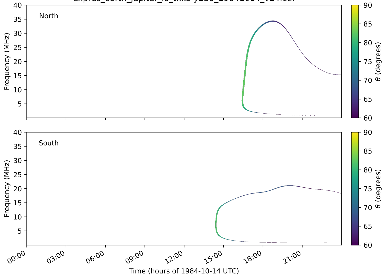
expres_earth_jupiter_io_txka-y235_19841014_v14.cdf
