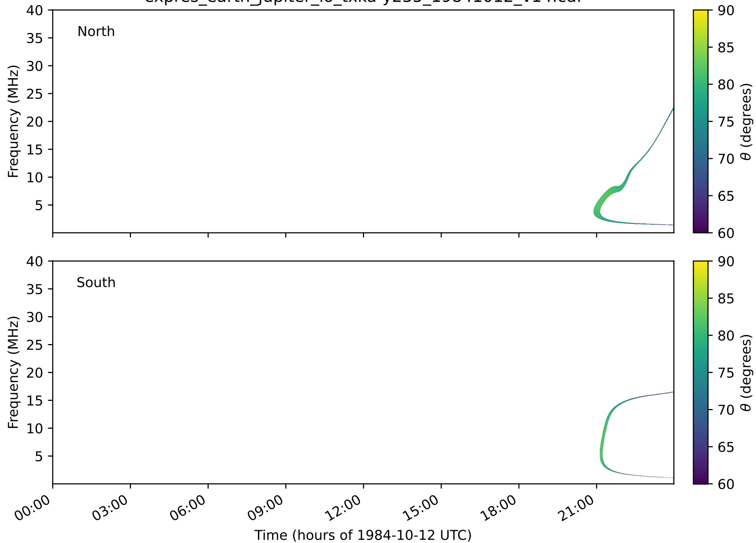
expres_earth_jupiter_io_txka-y235_19841012_v14.cdf
