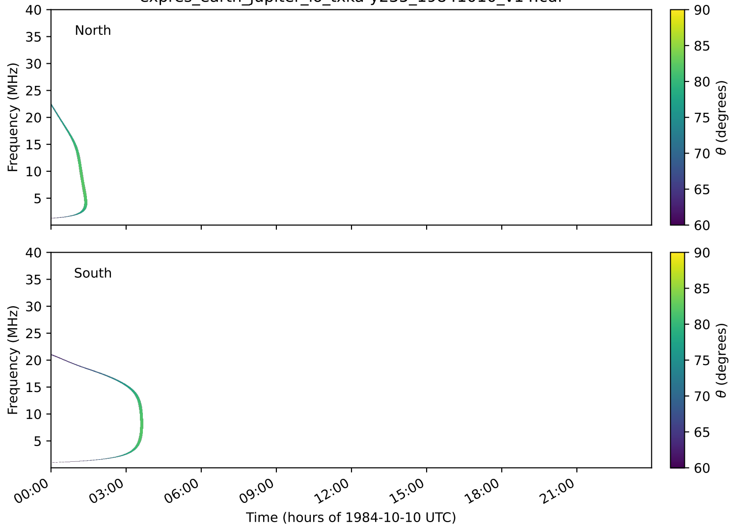
expres_earth_jupiter_io_txka-y235_19841010_v14.cdf
