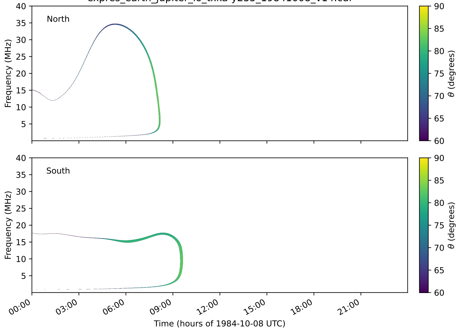
expres_earth_jupiter_io_txka-y235_19841008_v14.cdf
