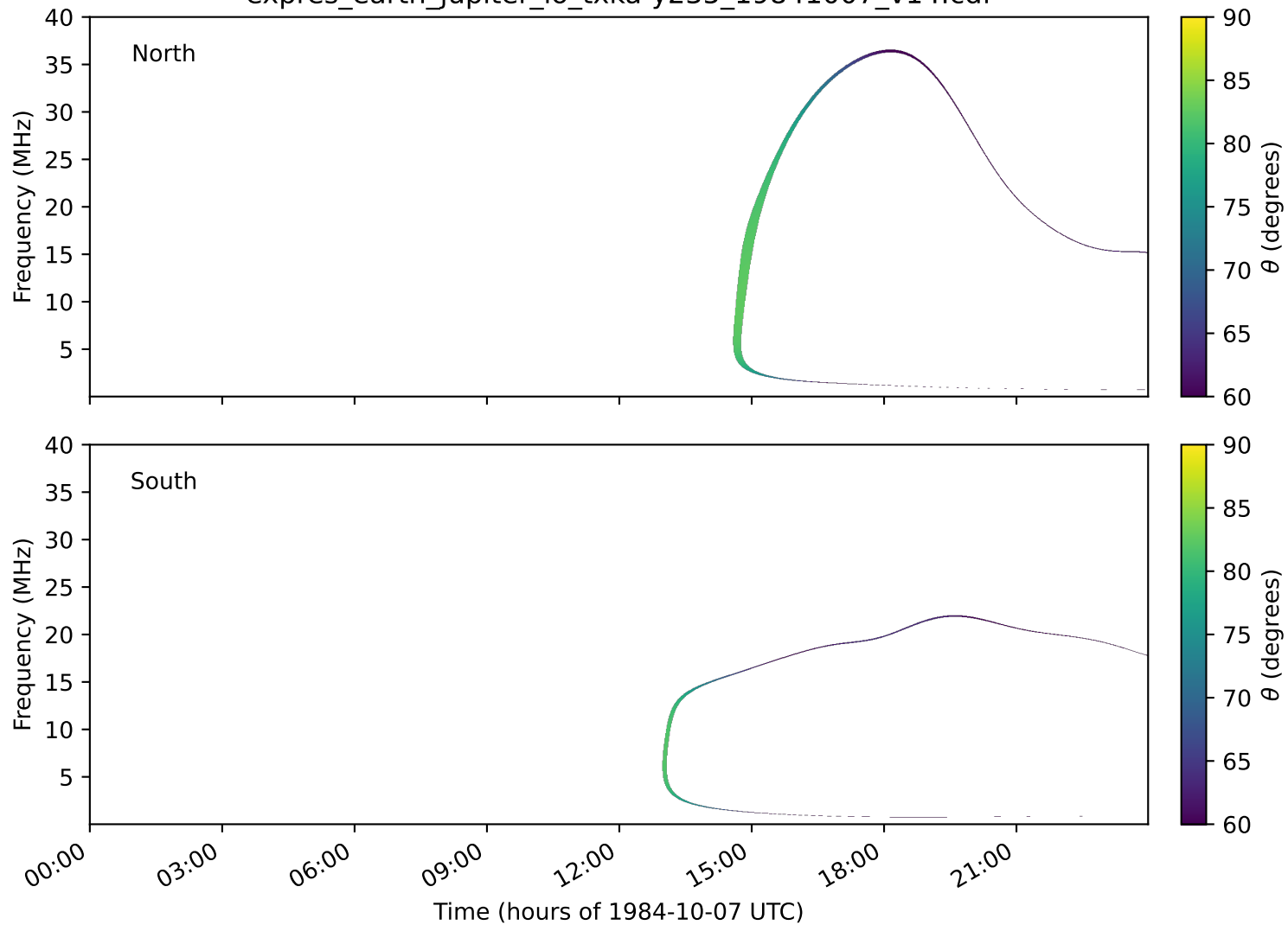
expres_earth_jupiter_io_txka-y235_19841007_v14.cdf
