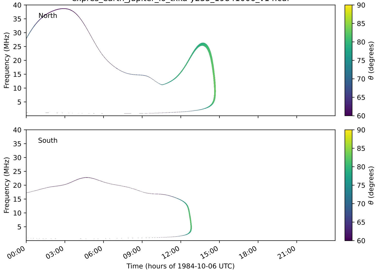
expres_earth_jupiter_io_txka-y235_19841006_v14.cdf
