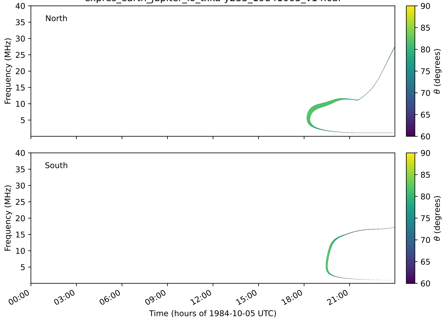
expres_earth_jupiter_io_txka-y235_19841005_v14.cdf
