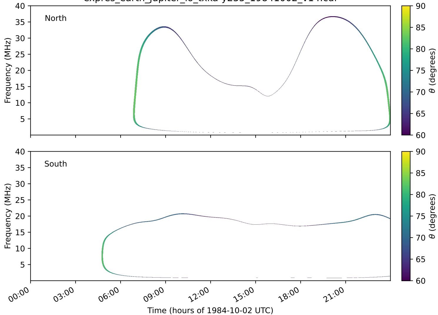
expres_earth_jupiter_io_txka-y235_19841002_v14.cdf
