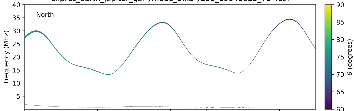
expres_earth_jupiter_ganymede_txka-y235_19841023_v14.cdf
