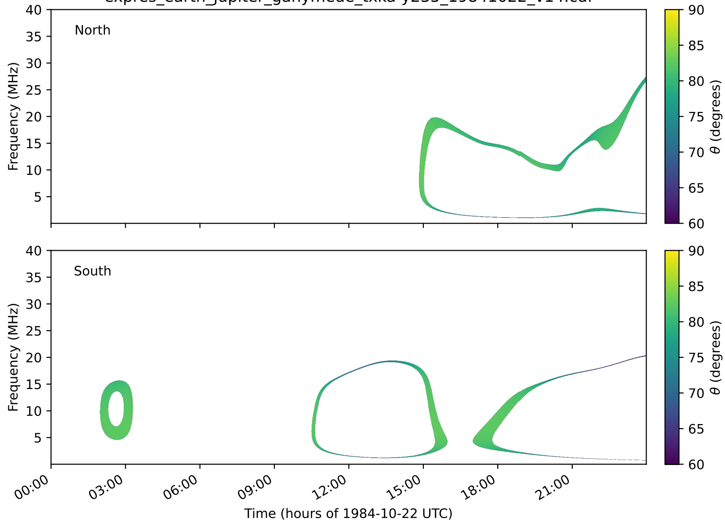
expres_earth_jupiter_ganymede_txka-y235_19841022_v14.cdf
