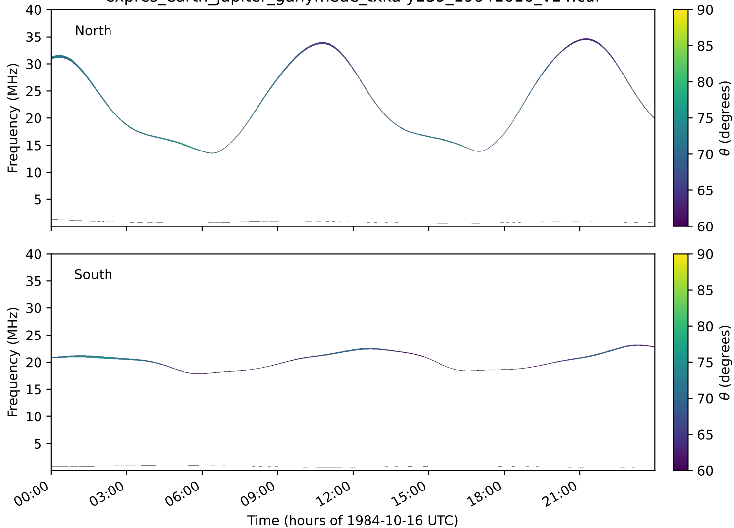
expres_earth_jupiter_ganymede_txka-y235_19841016_v14.cdf
